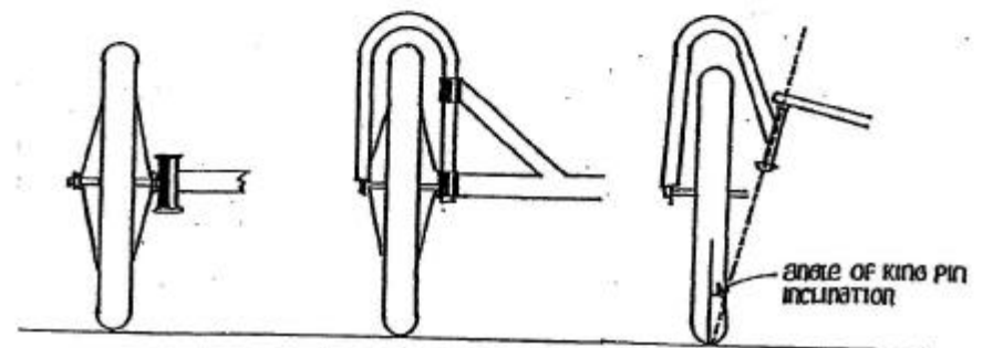
FIGURE 4 PRINCIPLE OF BOCKERMAN STEERING
